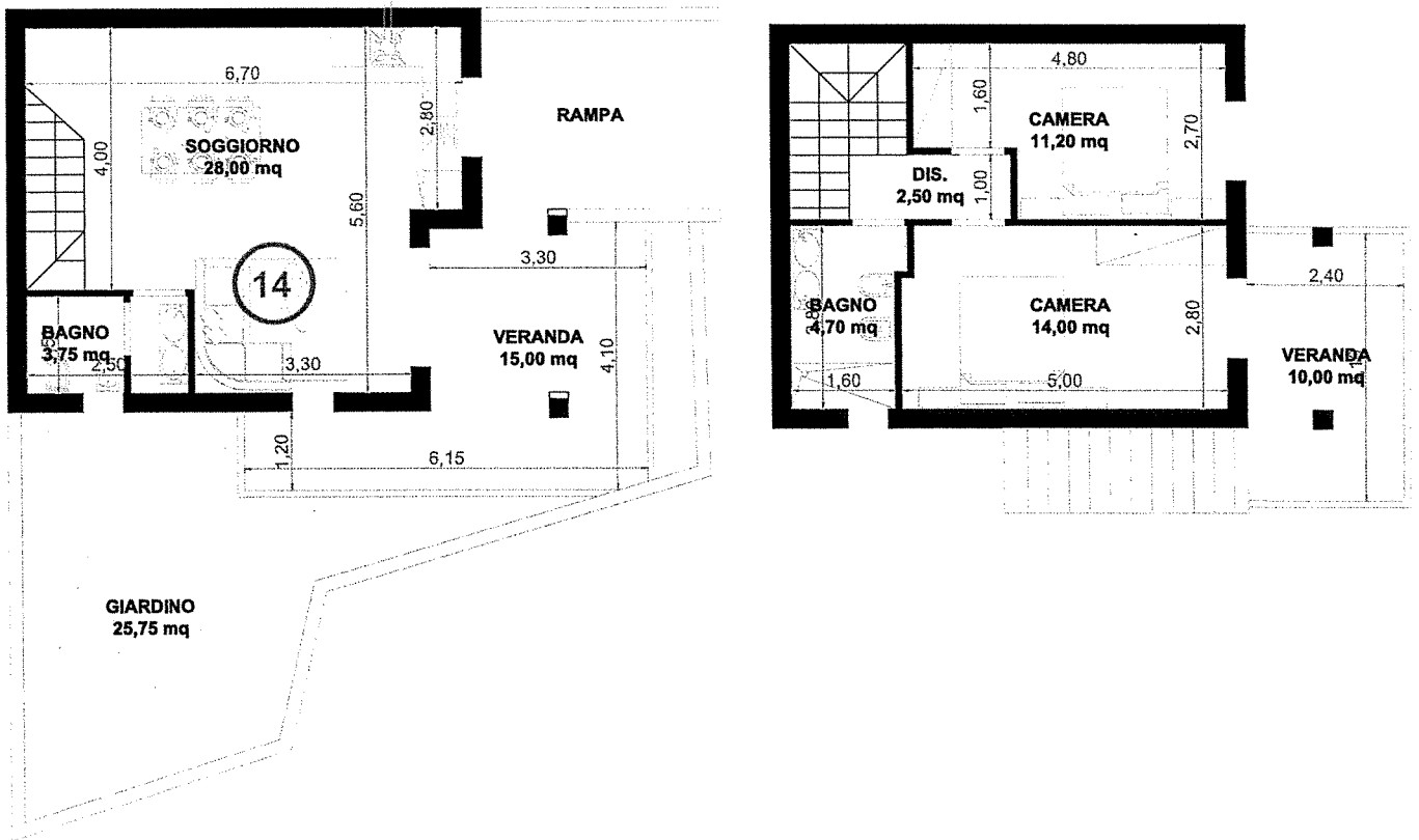
PIANO TERRA
